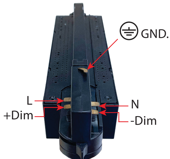
Dimmable & Tunable 4 Wires Track
