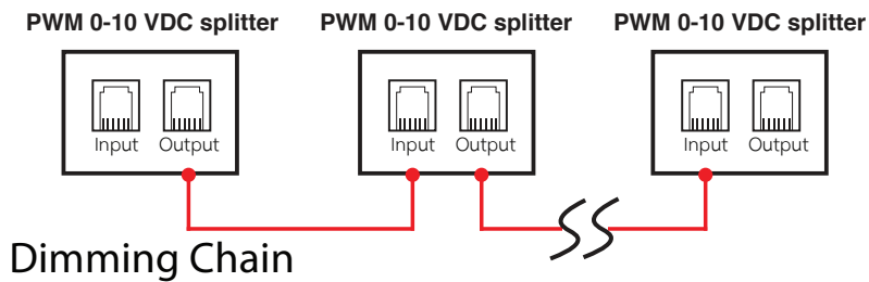
PWM 0-10 VDC Signal length 2 Meters
