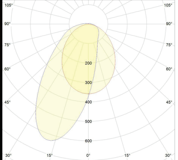
Asymmetric beam for wall washing
